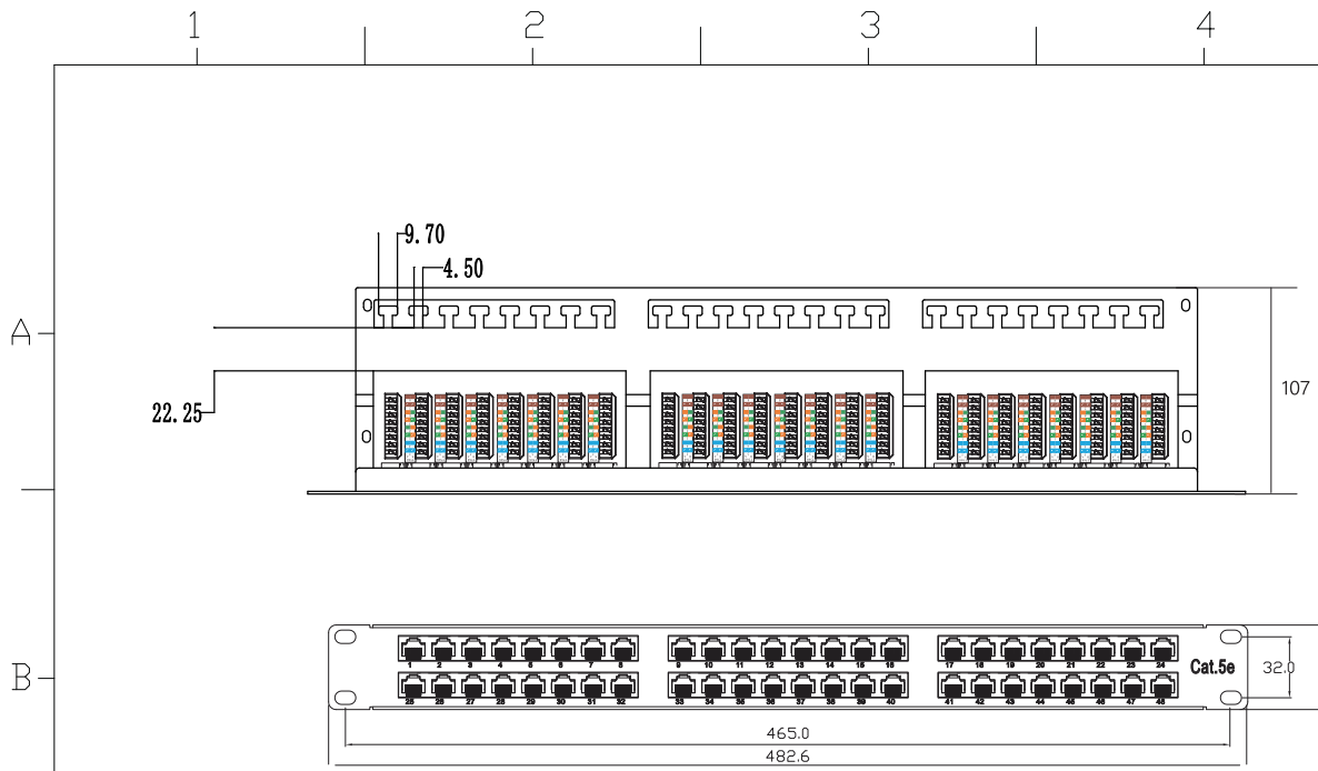
1u 19inch 48ports Cat5e FTP Patch Panel
